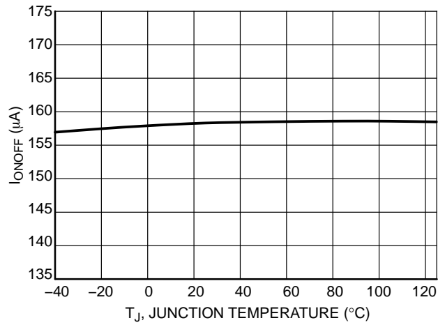
Figure 11. I_{ONOFF} at V_{CC} = 15\text{ V}
